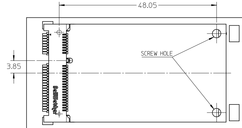
FULL-MINI CARD APPLICATION SCHEMATICS
